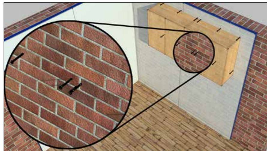
Fig. 9 Fixing kitchen units through Spacetherm Multi
