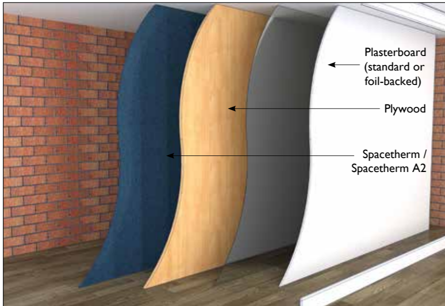
Fig. 1 Spacetherm Directfix / Spacetherm A2 Directfix Application
