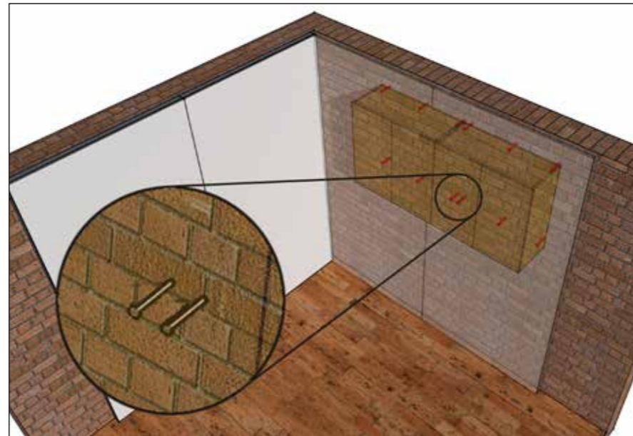
Fig. 9 Fixing kitchen units through Spacetherm Directfix / Spacetherm A2 Directfix
