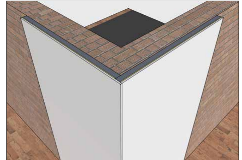
Fig. 5 External Angle Joint in Spacetherm Directfix / Spacetherm A2 Directfix
