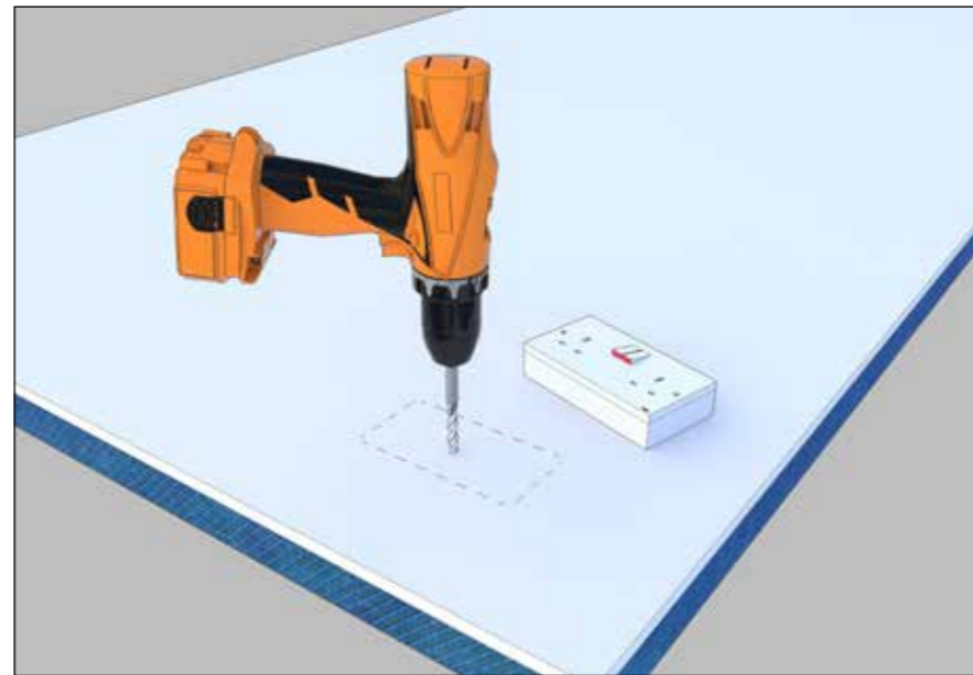
Fig. 3 Making cut-outs in Spacetherm Directfix / Spacetherm A2 Directfix
