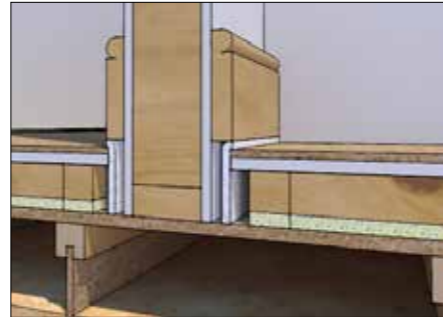
Fig. 5 Timber Installation
