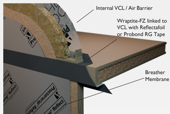
Cassette Floor Junction
