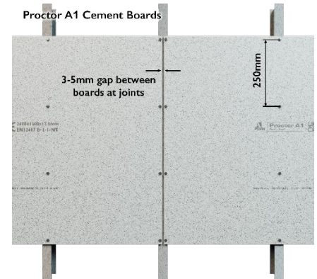
Diagram 3 - typical detail of fixing layout
