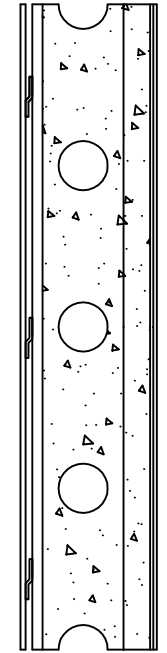
PROFLOOR MICRODECK – 17MM SCREED (80kg/M3 MIN) CONCRETE SLAB (PRECAST OR INSTU) RESILIENT CEILING SYSTEM ON TIMBER BATTEN
