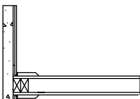
FLANKING/SUPPORT STRIP CUT BACK TO EDGE OF SKIRTING PROFLOOR MICRODECK – 17MM CONCRETE SUBFLOOR
