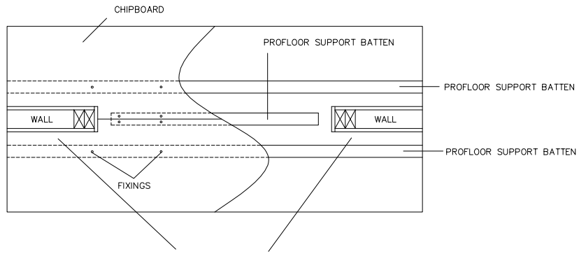
FLANKING STRIP AT ALL WALL PERIMETERS
