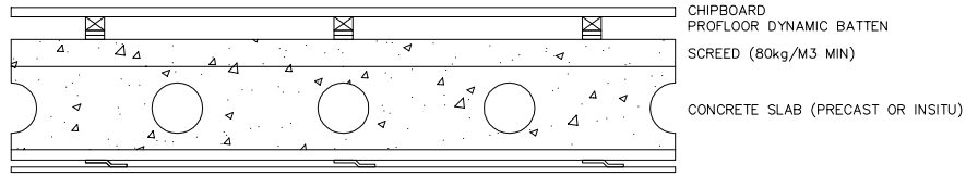
RESILIENT CEILING SYSTEM ON TIMBER BATTEN
